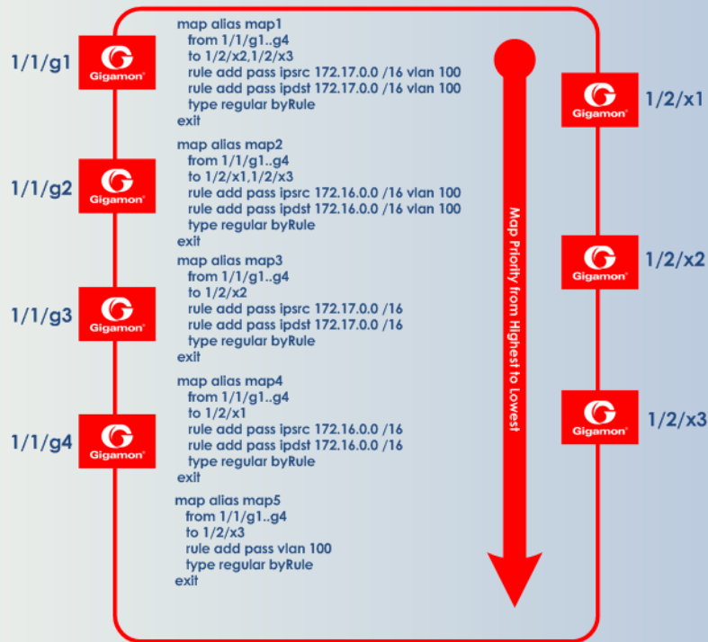
Figure 4 Sending Subnets and VLANs to Different Ports
