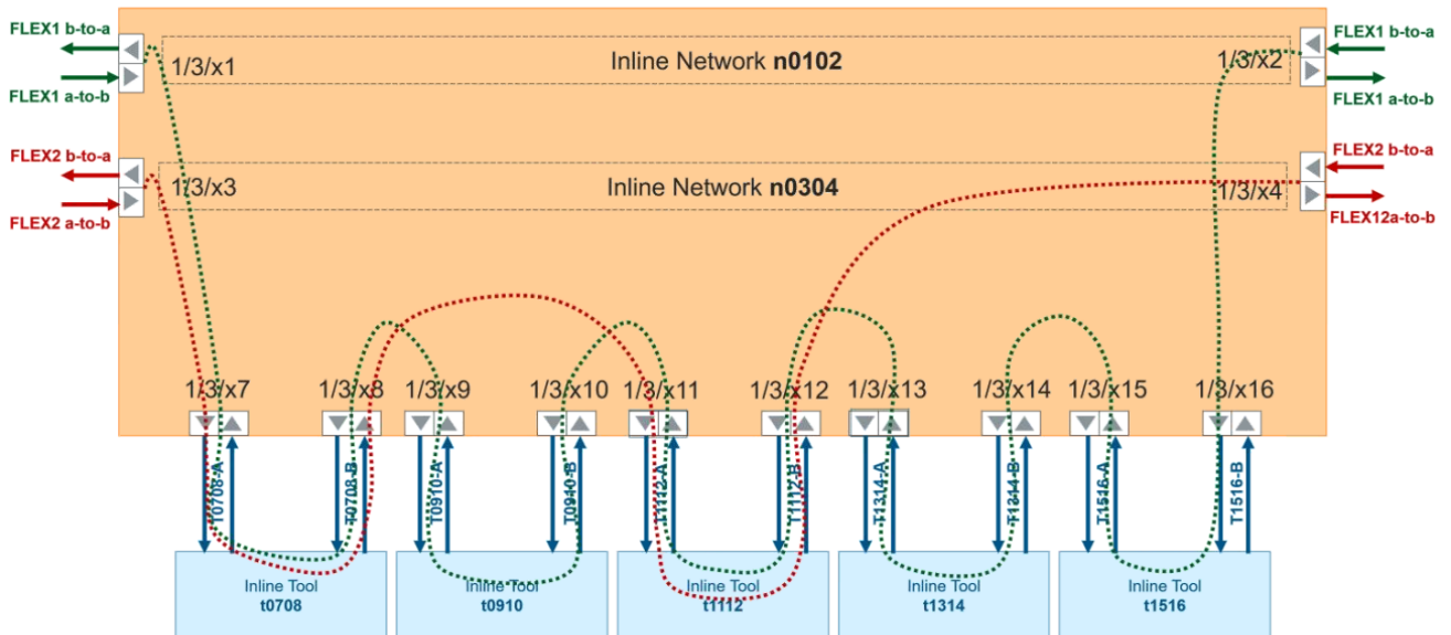
Figure 12 Example 2 Inline Tool Sharing by Multiple Inline Flows
